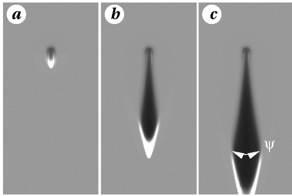
FIG. 3. Gray-coded images demonstrating evolution of triangular avalanche for t=50 (a), t=200 (b), and 250 (c). White shade corresponds to maximum height of the layer, and black to minimum height. Parameters of Eqs. (12) and (13) are, \alpha=0.15 , \beta=0.25 , \delta=1.2 , and h_0=3 .
