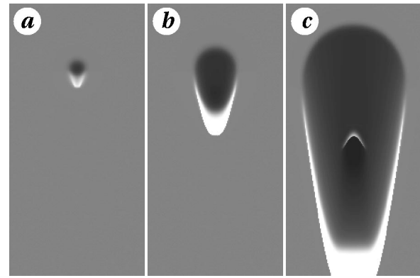
FIG. 4. Images of an up-hill avalanche for t=40 (a), t=100 (b), and 180 (c). Parameters of Eqs. (12) and (13) are, \alpha=0.05 , \beta=0.25 , \delta=1.07 , and h_0=5.5 . A small secondary avalanche is seen on the image (c).
