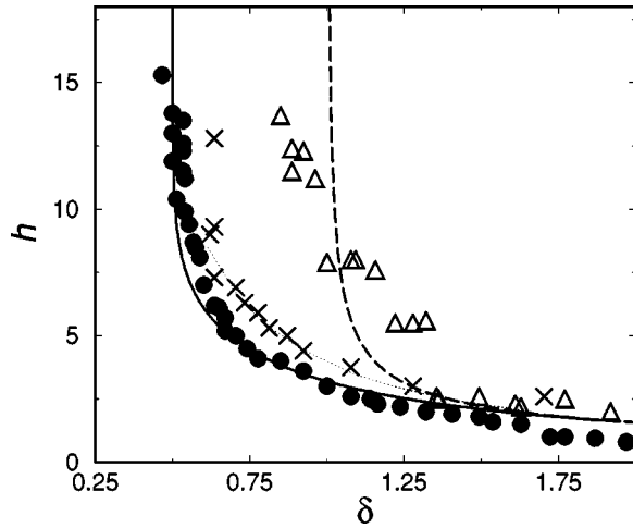
FIG. 2. Stability diagram. Dashed line shows the neutral curve [Eq. (7)], solid line shows the existence limit of fluidized state [Eq. (8)], dotted line shows the transition from triangular to up-hill avalanches for \beta=3.15 and \alpha=0.025 . Symbols show experimental data from Ref. [7].
